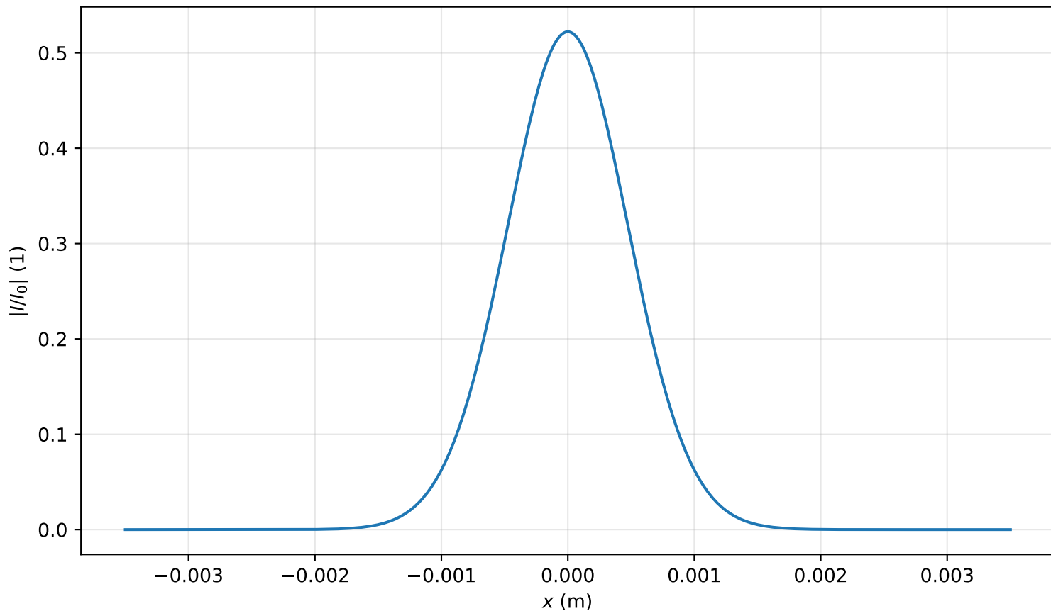
Intensity profile I(x, y = 0, z = 2.070m)/I_0 , P_{in}=0.1P_{cr} , artificial time
